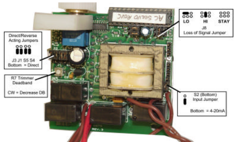
Fig. 1 Jumper Selections
